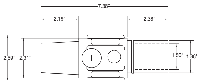
Female Connector
