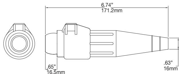
Female Connector
