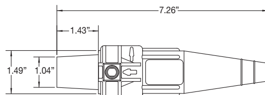
Female Connector
