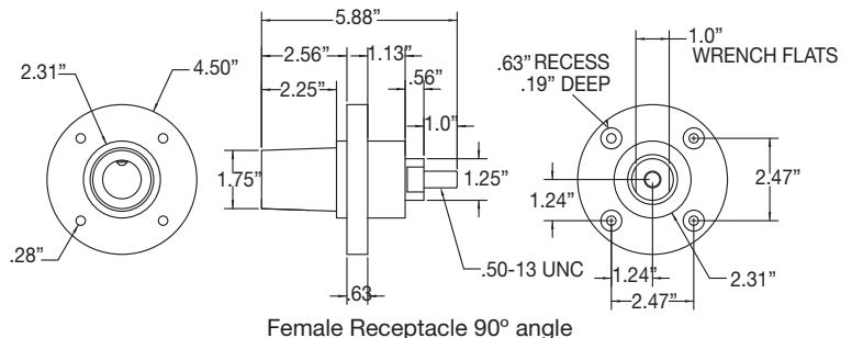
Female Receptacle 90° angle
