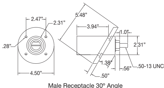
Male Receptacle 30° Angle
