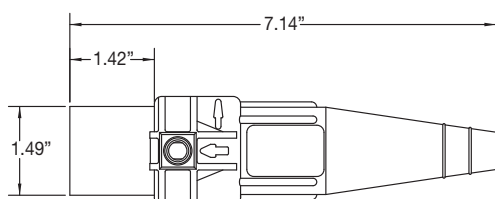
Male Connector
