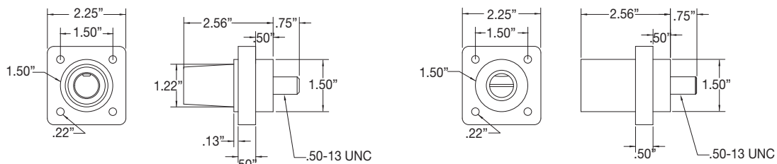
Female & Male E1016 Threaded Stud Receptacles, 3/4" Stud
