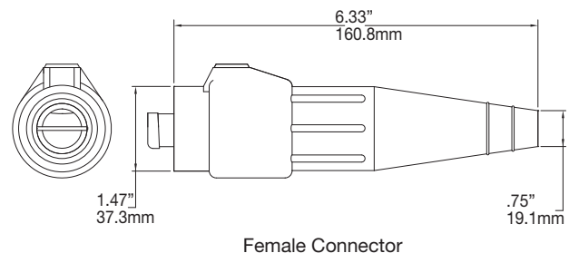
Female Connector
