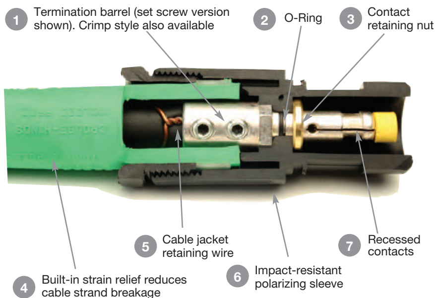
Cut-away view of E0200 male plug
