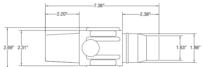
Female Connector
