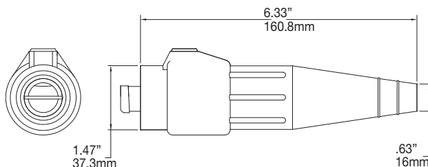
Male Connector
