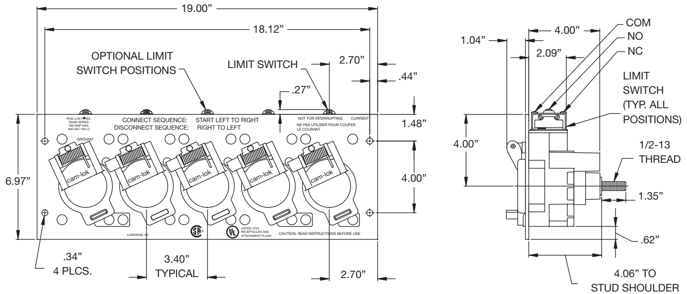
Cut-out and product dimensions/caps
