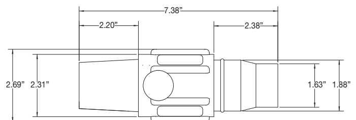
Female Connector
