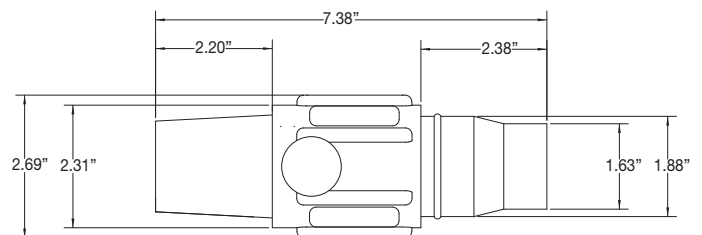
Female Connector
