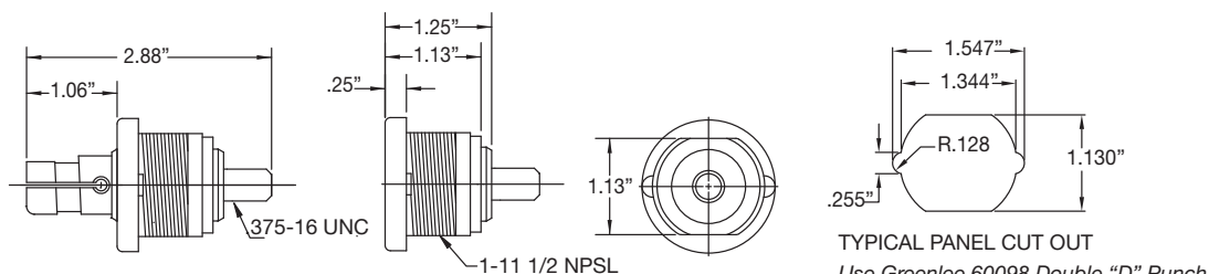
Male & Female High Temperature Receptacles
