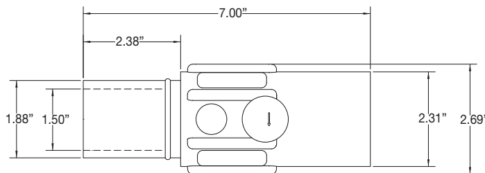
Male Connector
