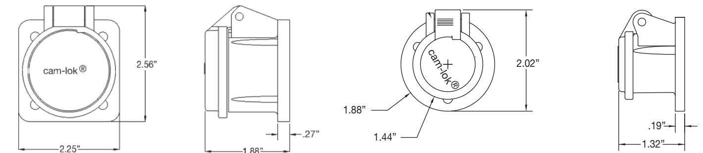
Snap Back Enclosure Assembly
