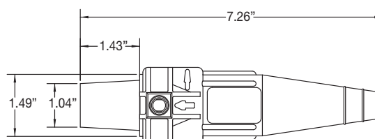
Female Connector
