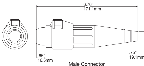
Male Connector
