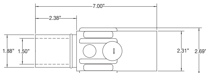
Male Connector
