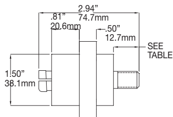
Male Receptacle
