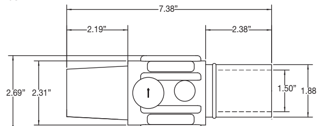
Female Connector
